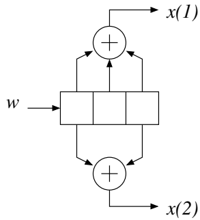
5, 7 Code Constraint Length 2
