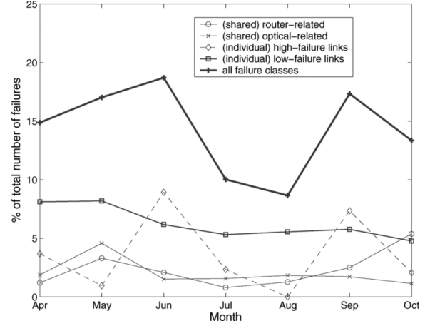
Fig. 14. Number of failures per month, per class and aggregate, (reported as the percentage of the total number of failures in the entire measurement period).
