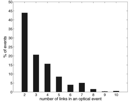
Fig. 10. Empirical pdf for the number of links in an optical event.
