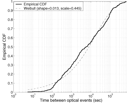
Fig. 11. CDF for the network-wide time between optical events.
