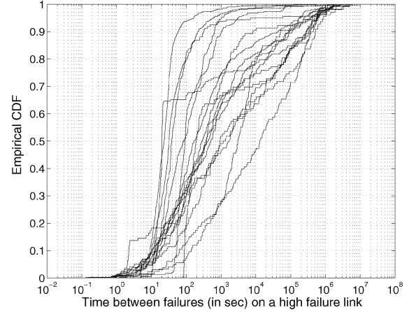
Fig. 12. Time between failures on each high failure link.
