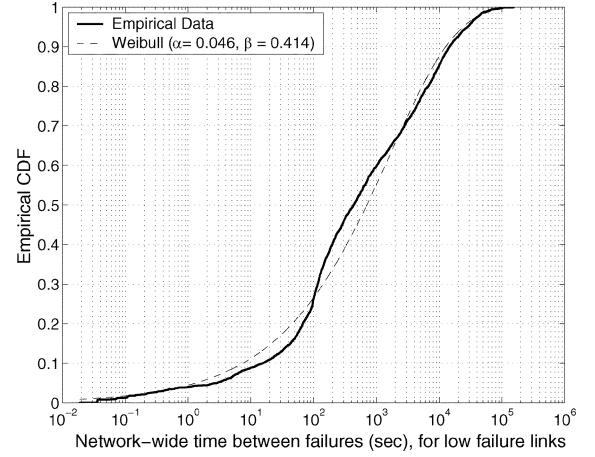
Fig. 13. Network-wide time between failures on low-failure links.
