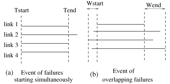
Fig. 3. Example events of simultaneous and overlapping failures. The time is according to the MRTD prepended at the IS-IS listener.
