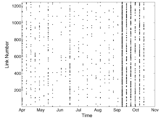
Fig. 6. Failures during weekly maintenance windows.
