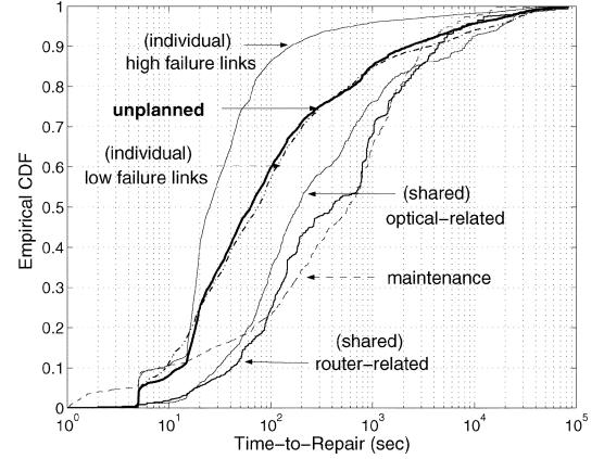
Fig. 5. CDF of the time-to-repair for each class of unplanned failures.
