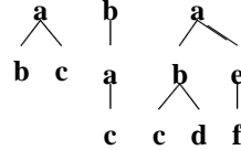
Fig. 1. Examples of tree strings: \mathbf{a}(\mathbf{b})(\mathbf{c}) , \mathbf{b}(\mathbf{a}(\mathbf{c})) , and \mathbf{a}(\mathbf{b}(\mathbf{c})(\mathbf{d}))(e(\mathbf{f})) , respectively.
